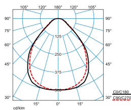
ArimoFit M73 PW19 42-8TW ETDD8 (DSU)
